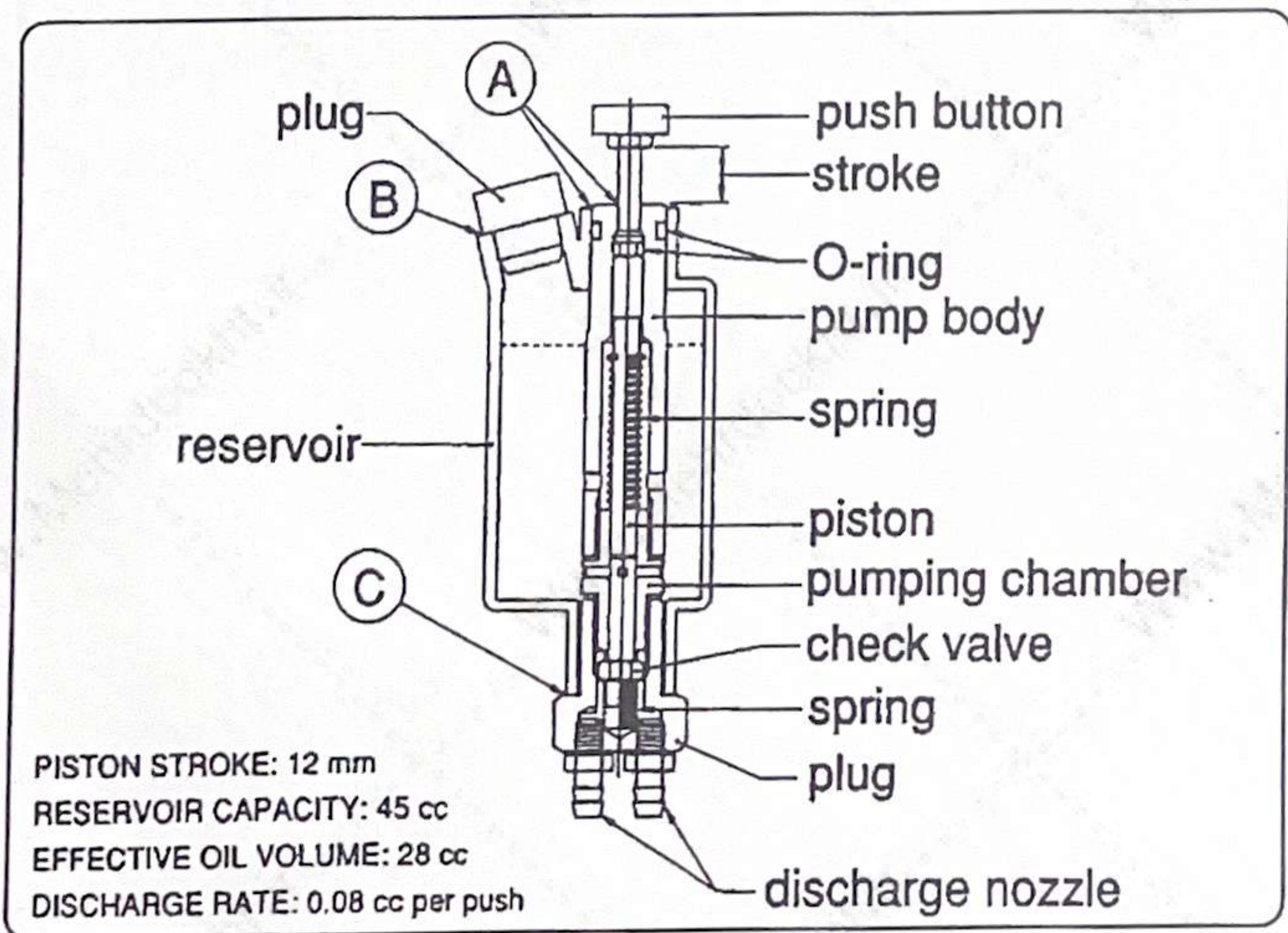
PUSH-BUTTON LUBRICATOR Model:NP-7A
